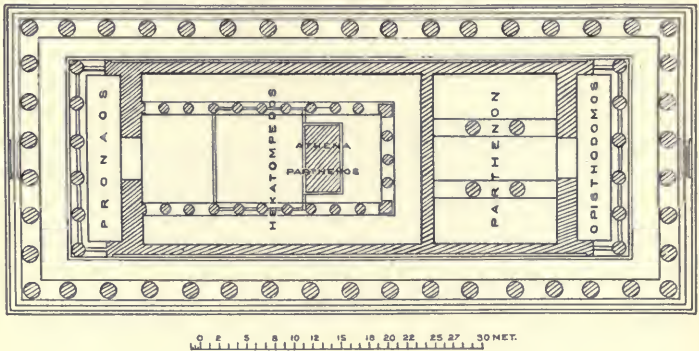
FIG. 13. — GROUND PLAN OF THE PARTHENON
